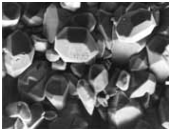
Before regeneration: sulfated battery
